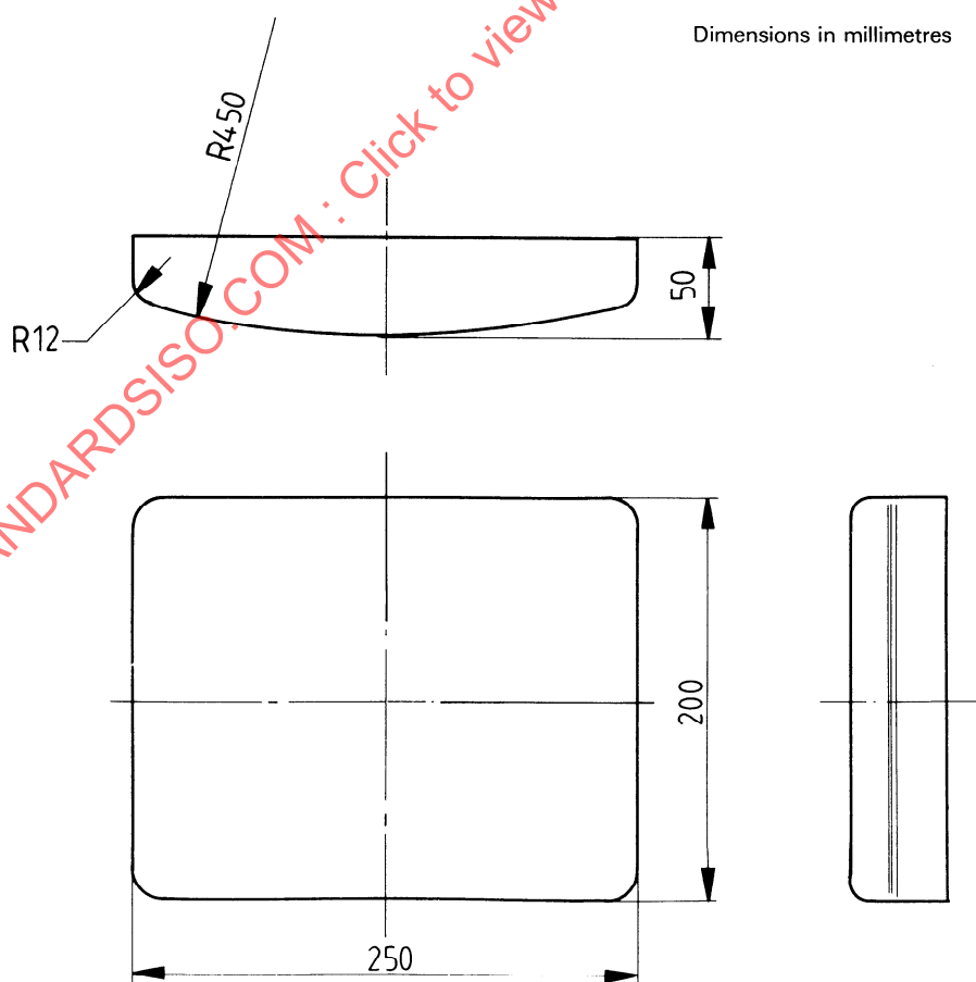
Figure 15 — Details of back loading pad
