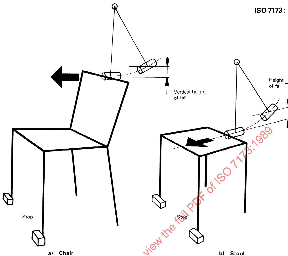
Figure 10 — Back impact test
