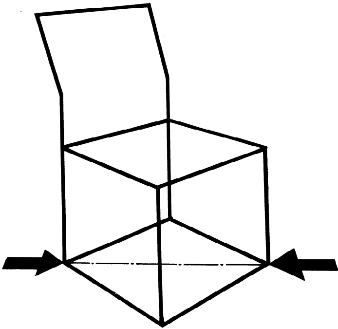
Figure 8 — Diagonal base load test — Directions of forces
