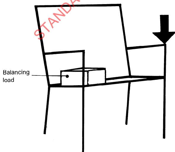
Figure 4 — Arm downwards static load test
