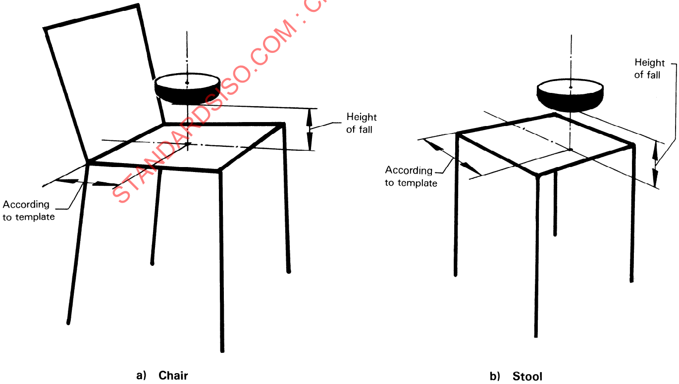
Figure 9 — Seat impact test
