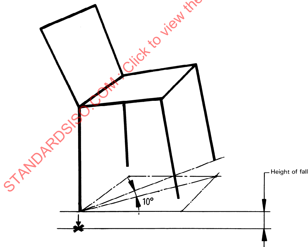
Figure 12 — Drop test
