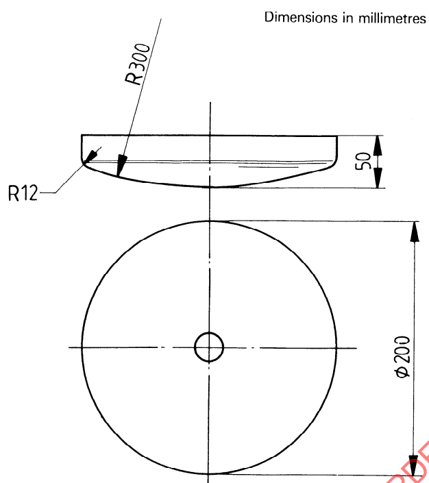
Figure 14 — Details of the smaller seat loading pad
