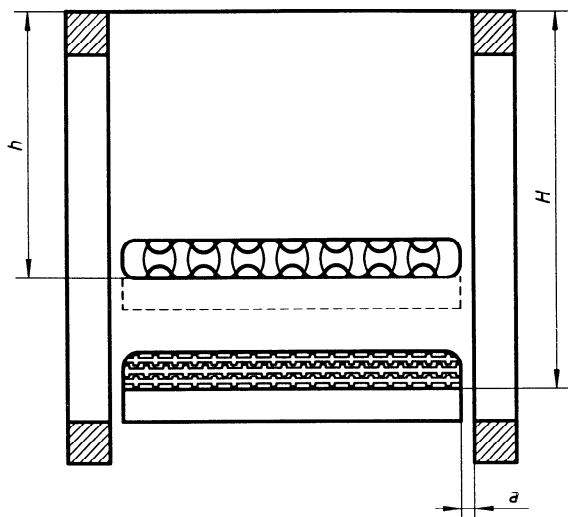
Figure A.1 — Cross section
