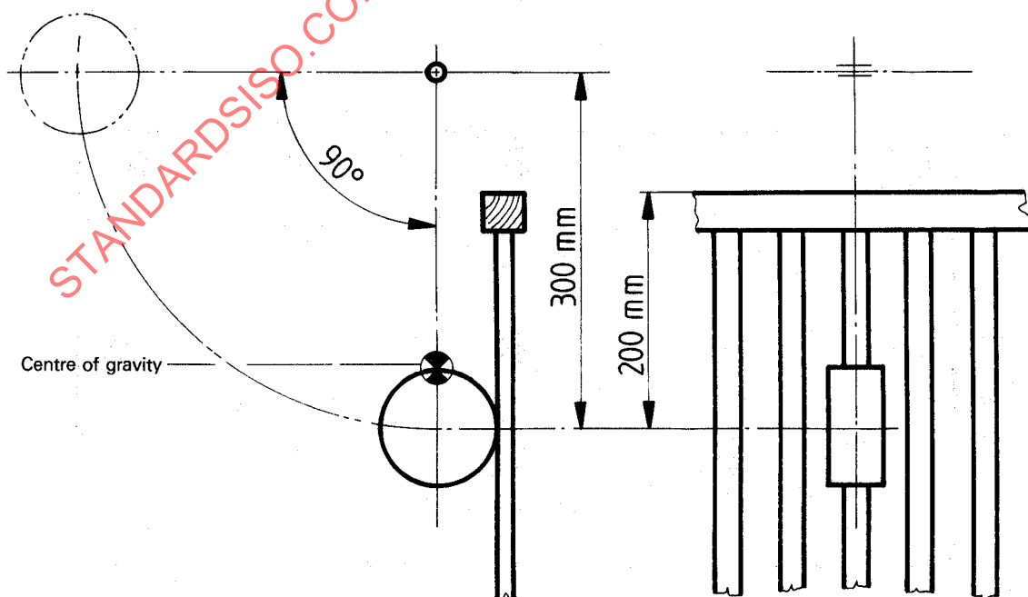
Figure 4 — Side impact pendulum
