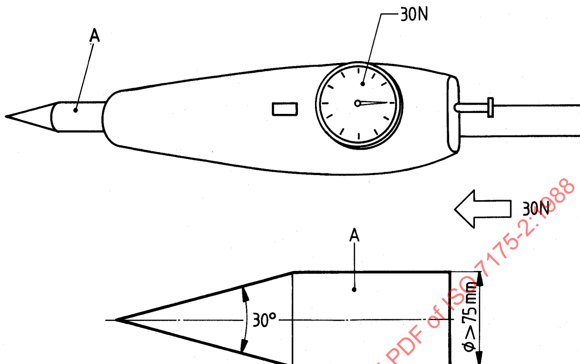
Figure 1 — Example of measuring cone
