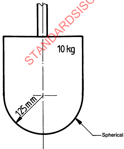
Figure 2 — Bottom impactor
