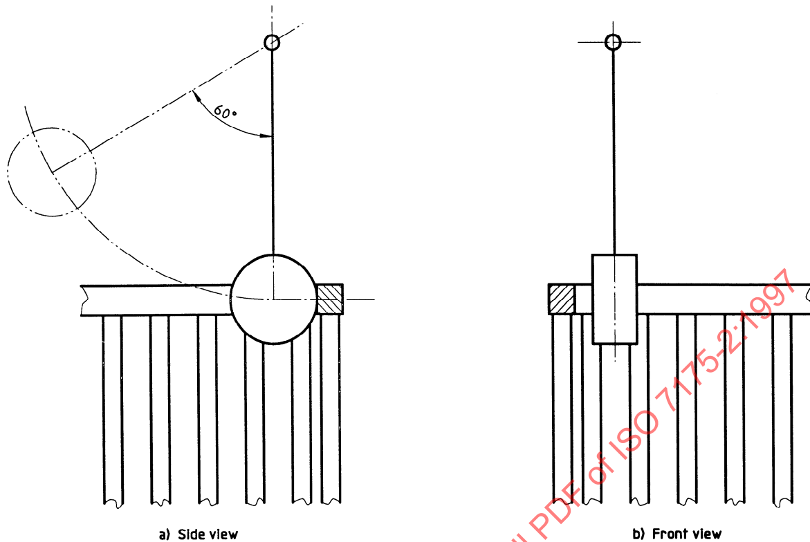
Figure 10 — Corner impact test
