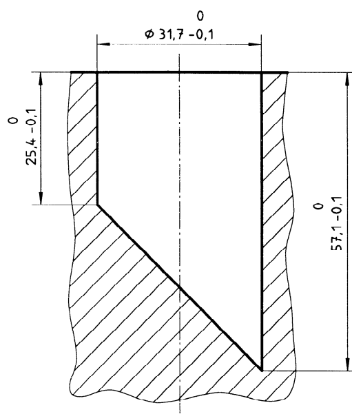
Figure 7 — Cylinder
