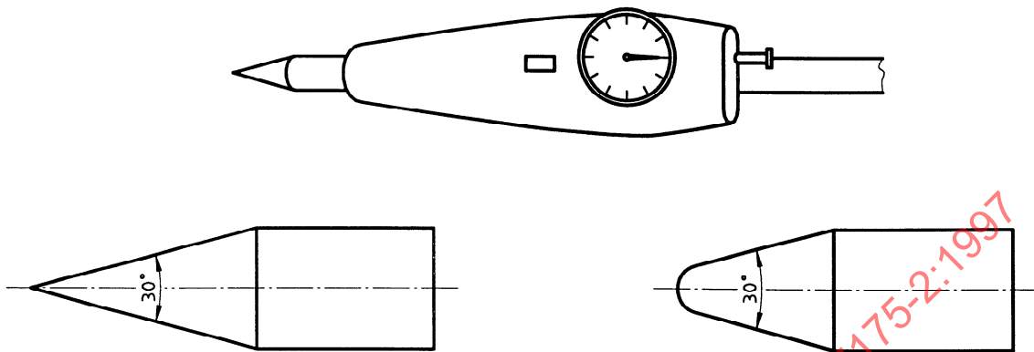
Figure 1 — Examples of measuring cones
