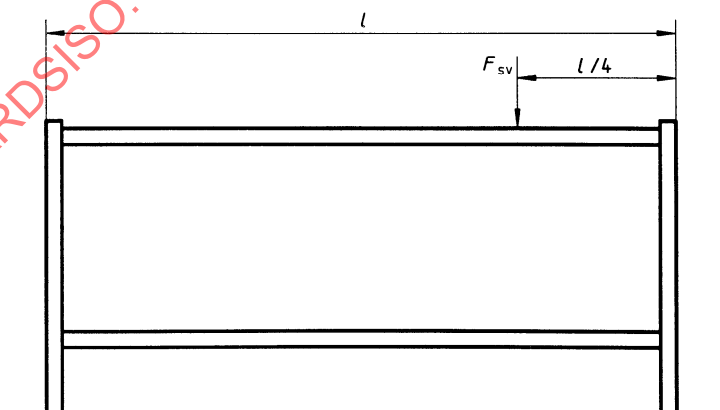
Figure 11 — Vertical static load test
