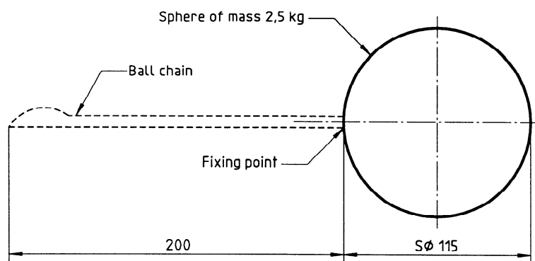
Figure 5 — Test chain with loop
