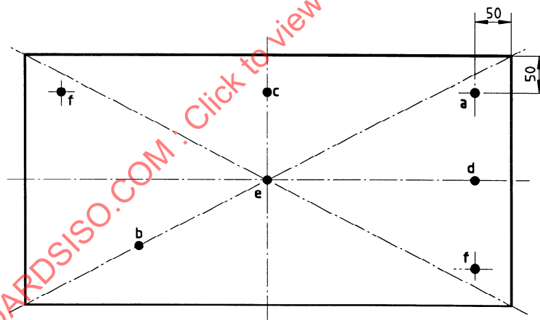
Figure 8 — Impact points
