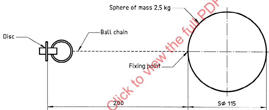
a) Test chain with disc
