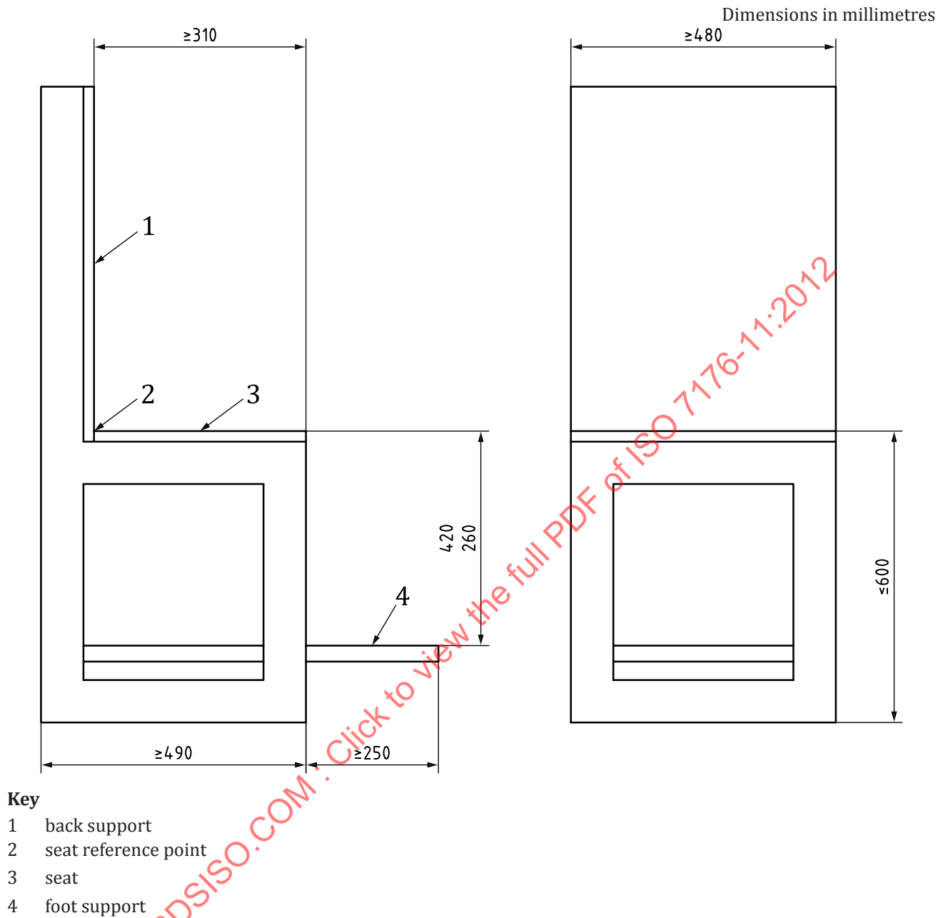
Figure 1 — Test fixture
