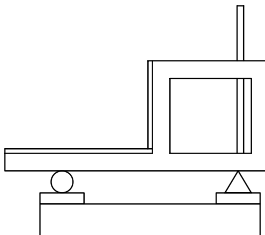
Figure A.5 — Empty test fixture lying on scales
