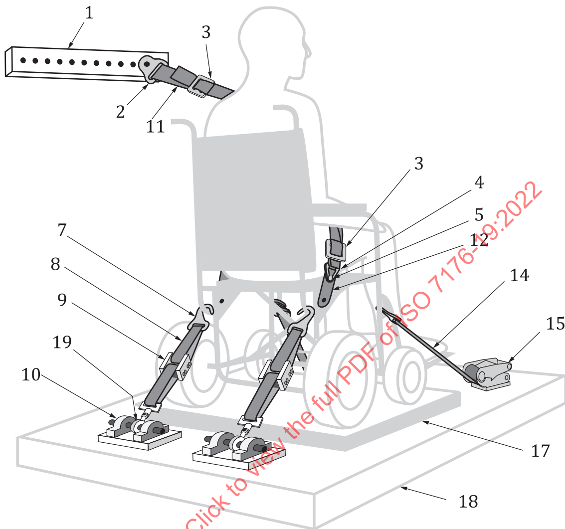
b) Rear-oblique view drawing of SWTORS with a surrogate shoulder belt and a wheelchair-mounted pelvic-belt restraint
