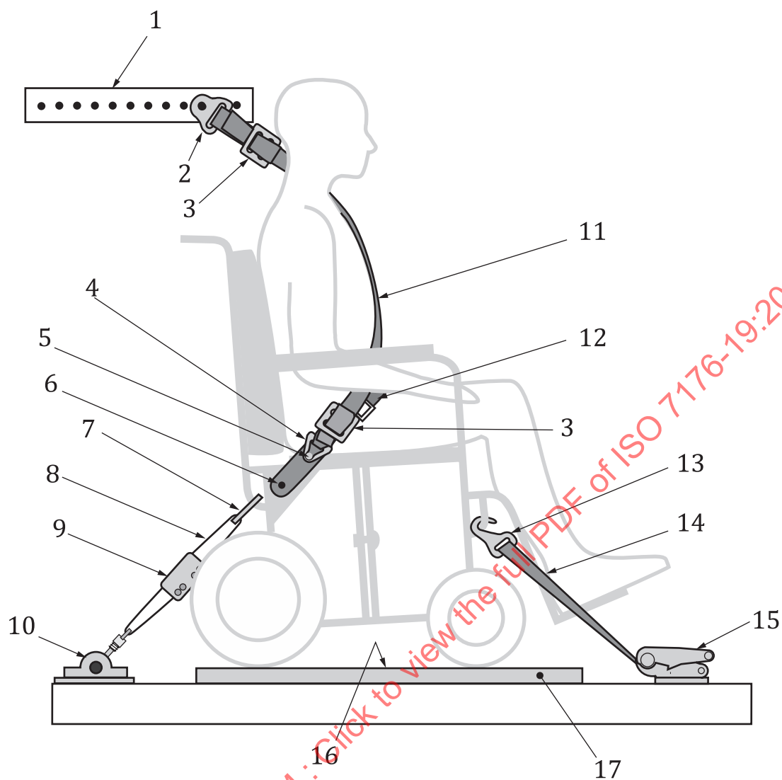
a) Side-view drawing of SWTORS with a surrogate shoulder belt and a wheelchair-mounted pelvic-belt restraint
