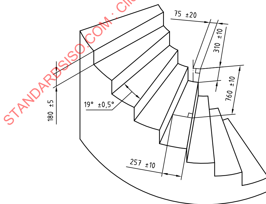
Figure 2 — Winding test stair (see 4.1.2)
