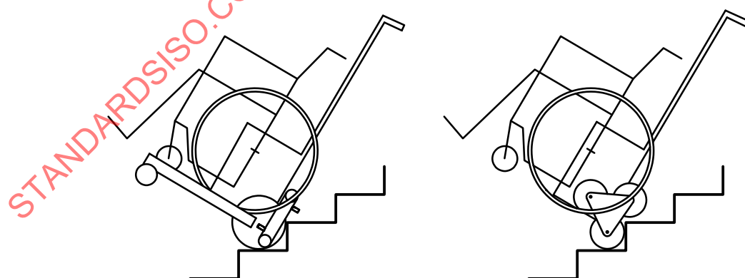
Figure A.4 — Representations of typical assistant-operated, manually stabilized stair-climbing wheelchair carriers (Type D)
