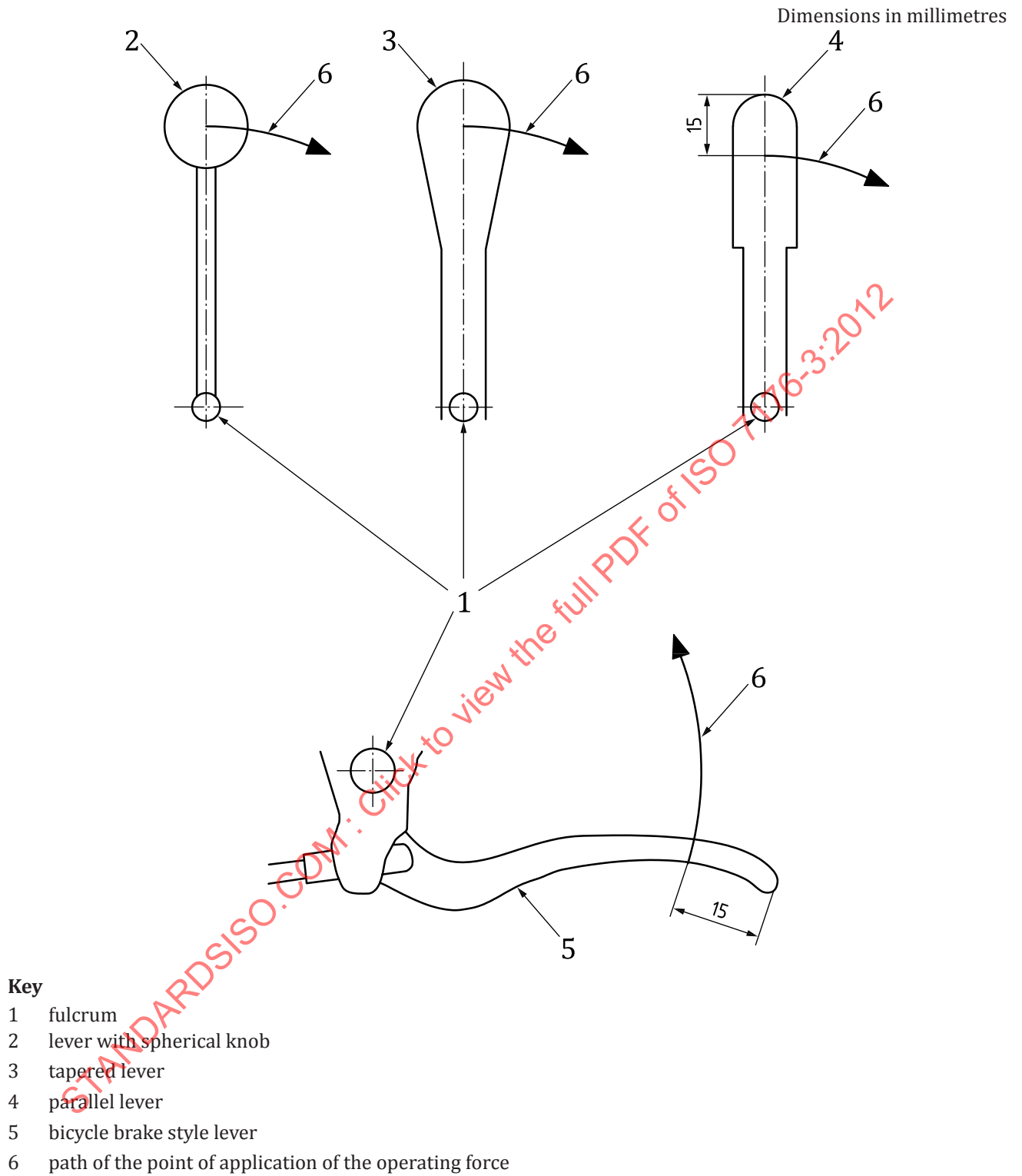
Figure A.1 — Application of force on hand-operated brakes
