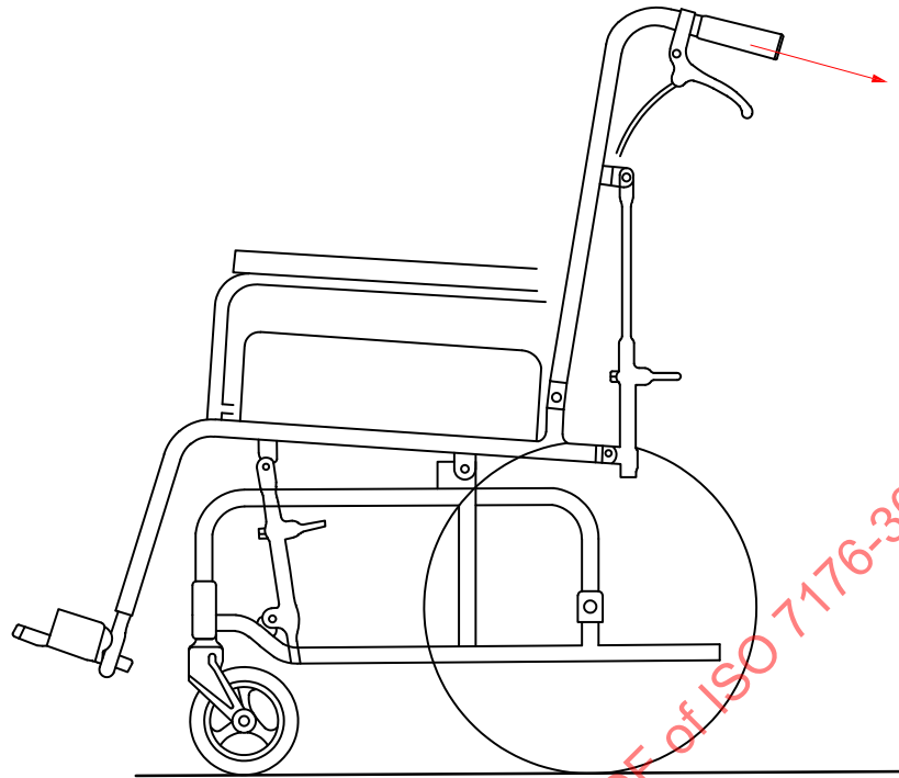
Figure 2 — Repeat test of raising the casters
