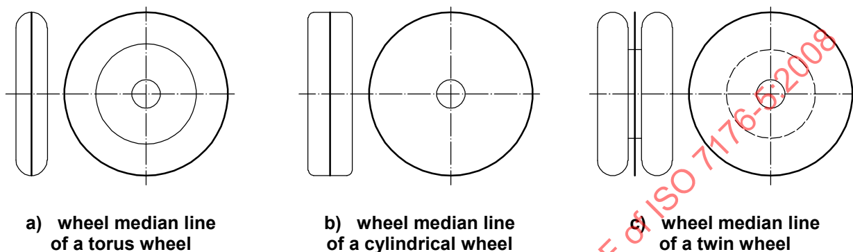
Figure 19 — Wheel median line
