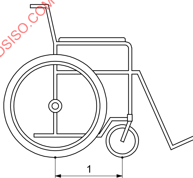
Figure 20 — Wheelbase
