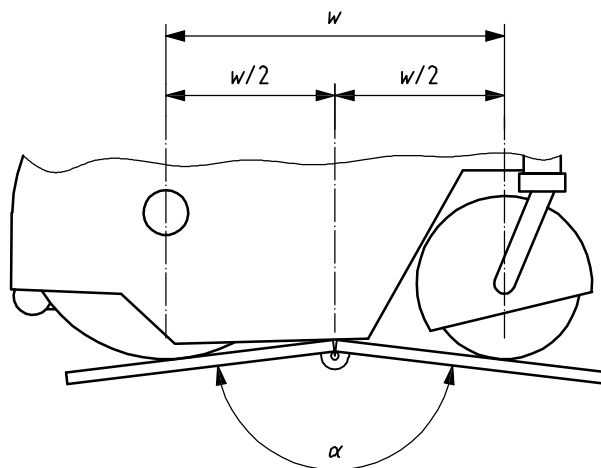
Figure A.2 — Measurement of greatest angle, \alpha , when wheelchair is at upper transition
