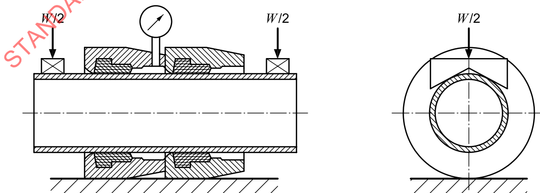
Figure 2 — Leaktightness of joints — External pressure
