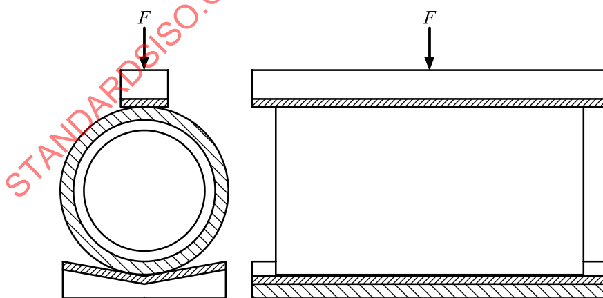
Figure 3 — Diametral stiffness test
