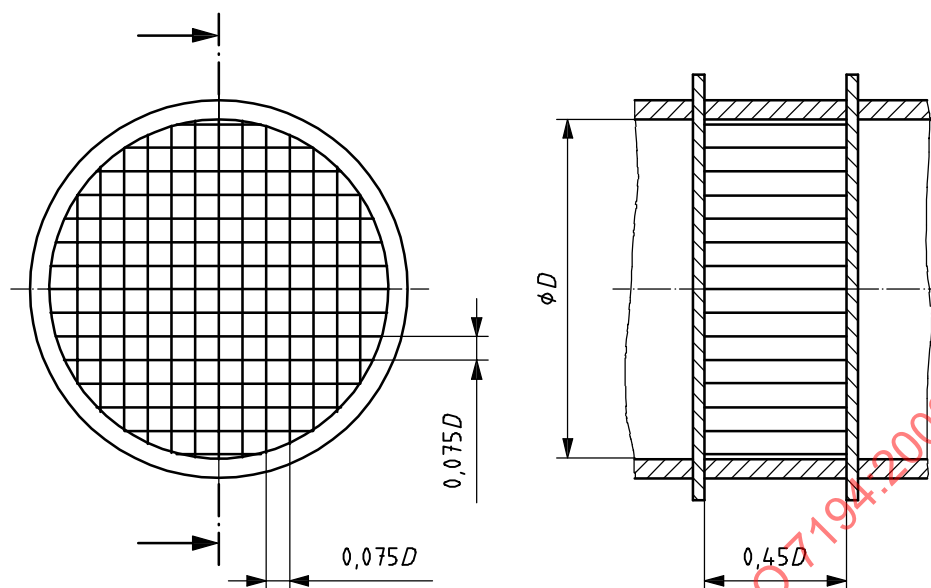
Figure 5 — Type D — AMCA straightener
