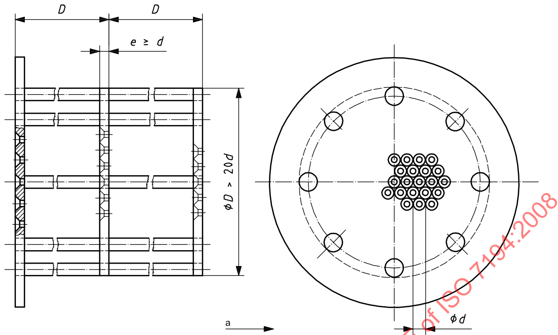
Figure 3 — Type B — Sprengle straightener (perforated plates)
