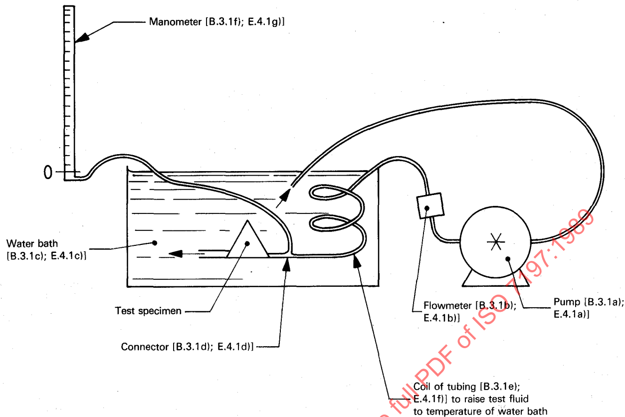
Figure B.1 — Example of a test rig for determining pressure and flow characteristics (see annex B) and durability (see annex E) of shunts and components
