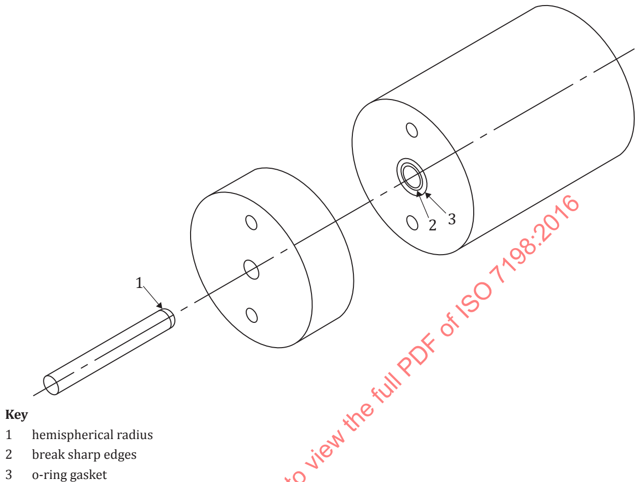
Figure A.2 — Example of a probe burst tester
