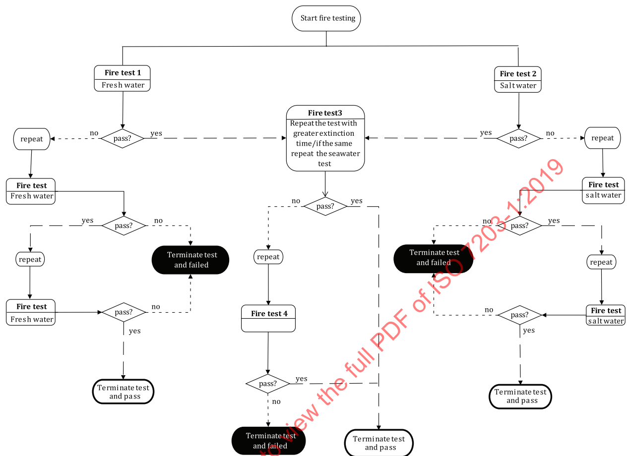
Figure G.1 — Decision tree for fire performance test on water-immiscible fuels
