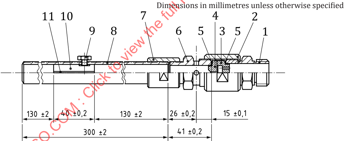
Figure F.2 — Foam collector for expansion and drainage measurement
