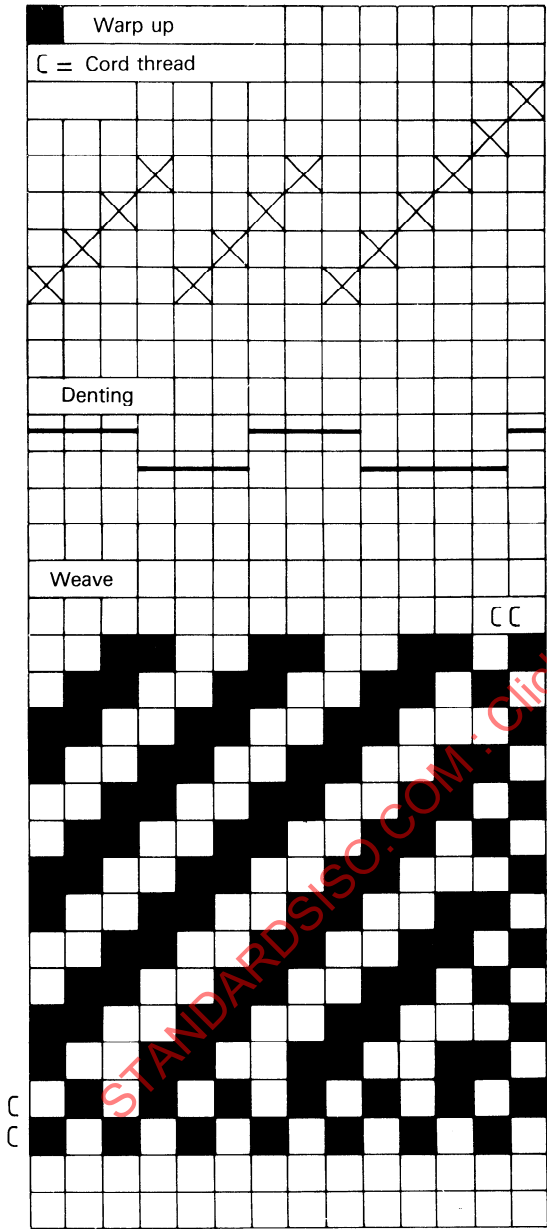
Figure 2a) — Drafting and denting plans of simple weave repeat
