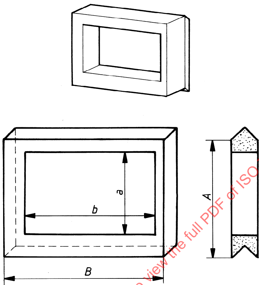
Figure 10 — Aperture bricks for square and rectangular windows
