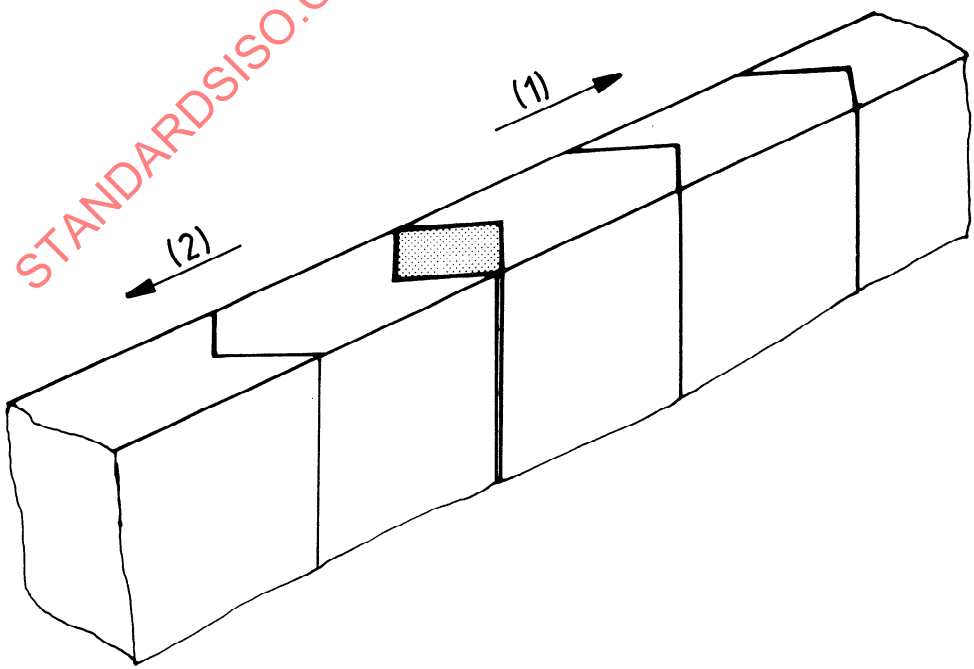
Figure 5 — Assembly of category 1 square bricks
