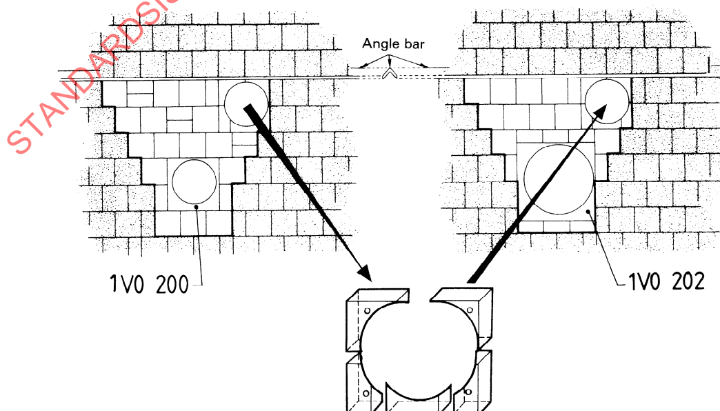
Figure 11c) — Example of use : replacement of a 1V0 200 aperture brick by a 1V0 202 aperture brick
