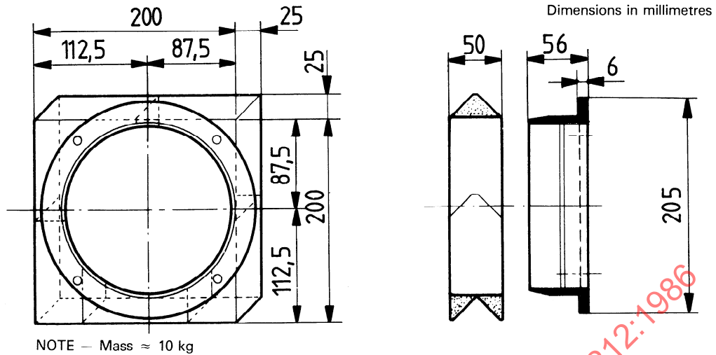
Figure 11a) — Special demountable circular aperture brick (1V0 220)
