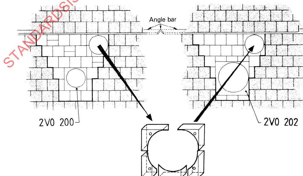
Figure 28c) — Example for use : replacement of a 2V0 200 aperture brick by a 2V0 202 aperture brick
