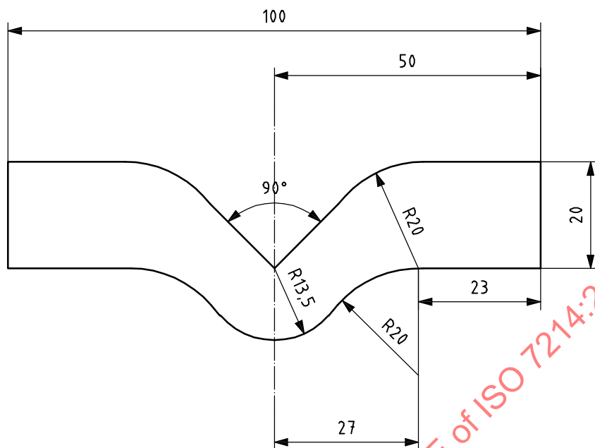
Figure 1 — Specimen for tear strength
