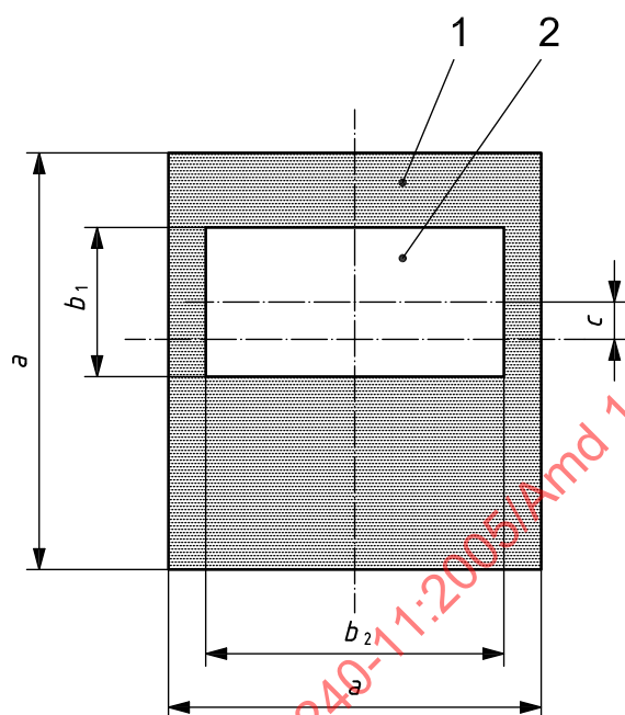
b) Example of a rectangular operating face
