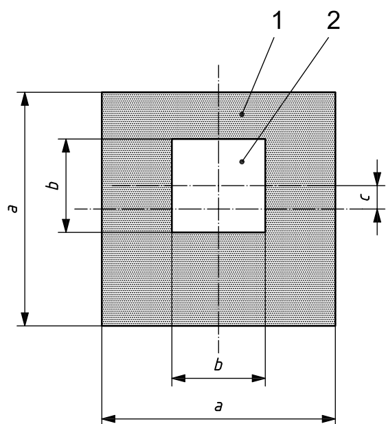
a) Example of a square operating face
