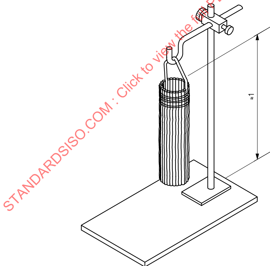
Figure E.1 — Arrangement of cotton wicks
