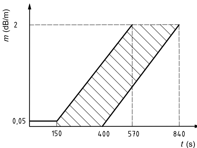
Figure D.3 — Limits for m against time, t , Fire TF2
