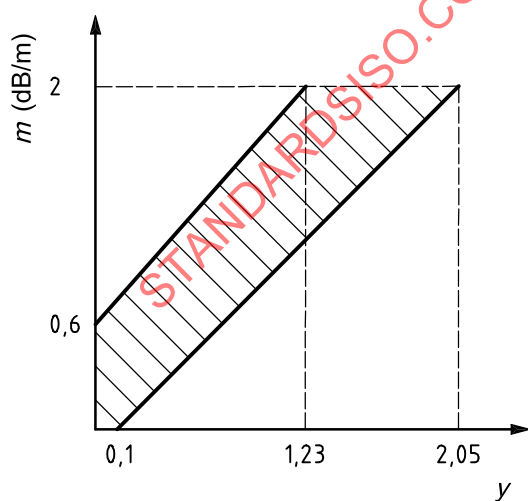
Figure D.2 — Limits for m against y , Fire TF2
