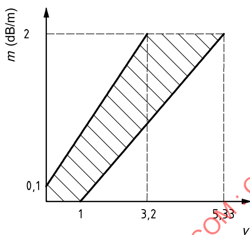
Figure E.2 — Limits for m against y , Fire TF3
