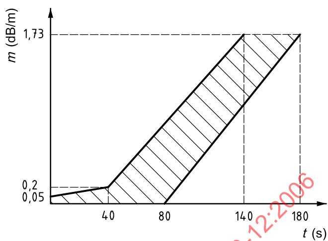
Figure F.2 — Limits for m against time, t , Fire TF4
