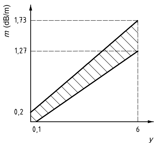
Figure F.1 — Limits for m against y , Fire TF4
