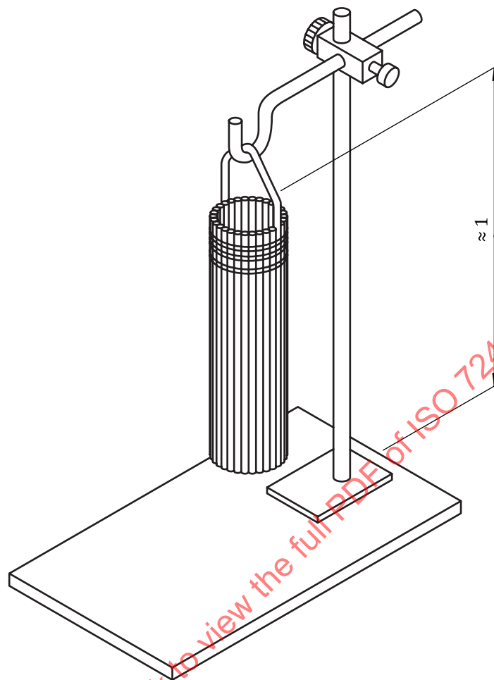
Figure E.1 — Arrangement of cotton wicks
