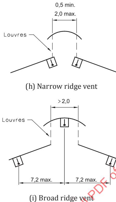
Figure 9 — Examples of point-type and line-type heat detector locations at ceiling, roof, or surface apexes
