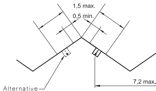
(c) Equal sloping surface
