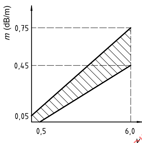
Figure H.2 — Limits for m against y , Fire TF1
