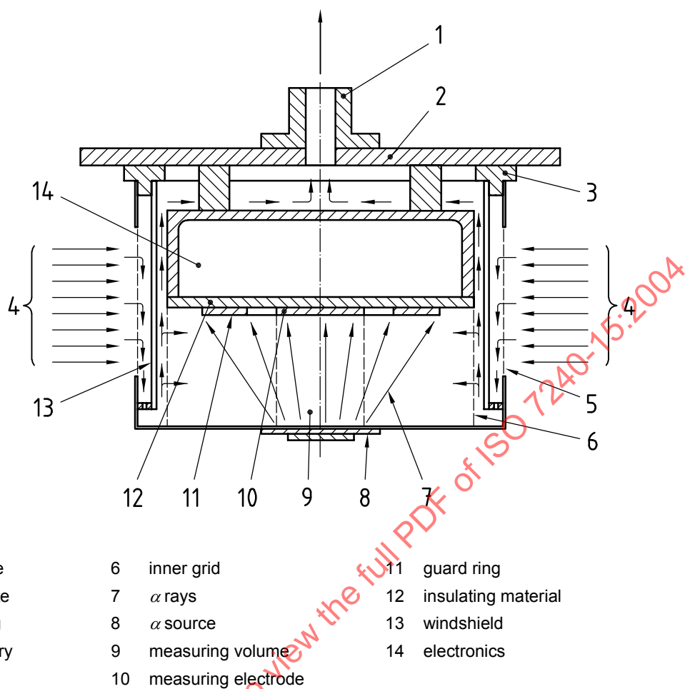
Figure A.2 — Measuring ionization chamber — Method of operation
