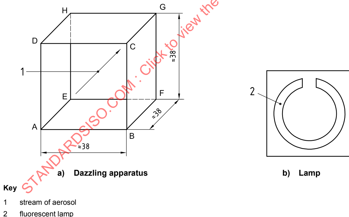
Figure E.1 — Dazzling apparatus a) and lamp b)
