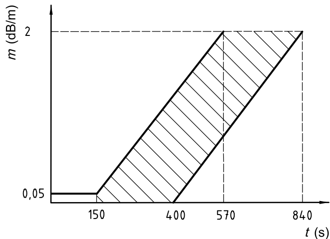
Figure I.3 — Limits for m against time, t , Fire TF2
