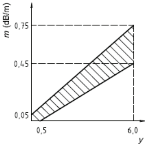
Figure G.2 — Limits for m against y , Fire TF1
