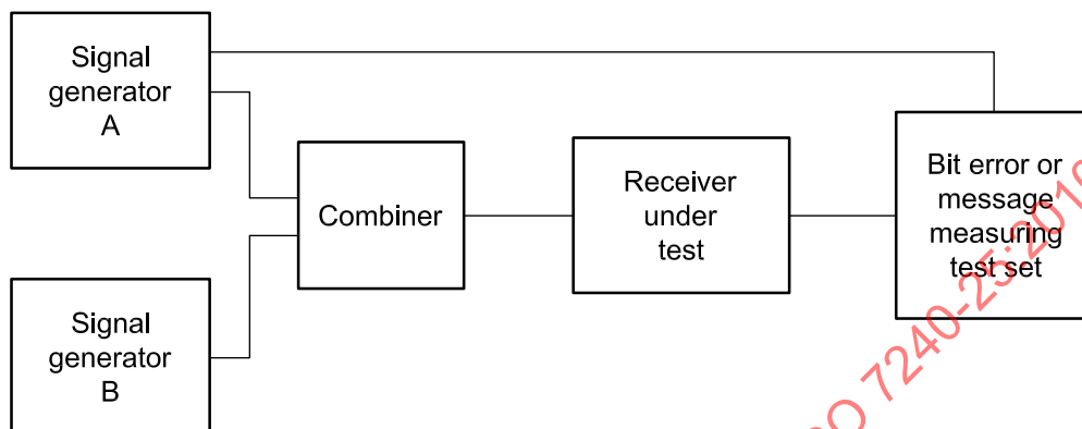
Figure 1 — Measurement arrangement
