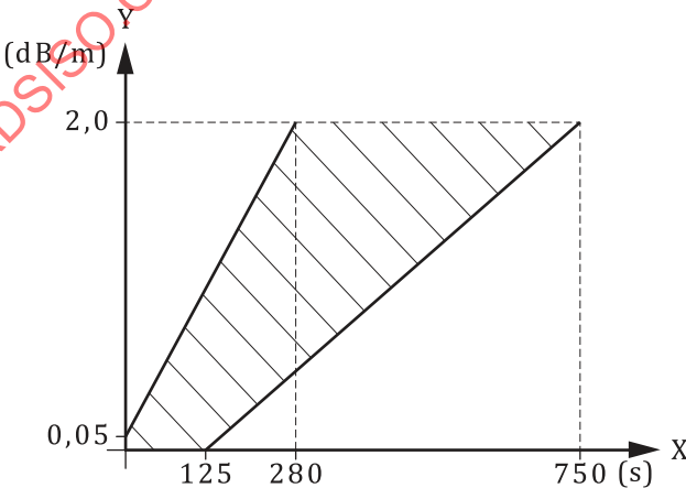
Figure H.2 — Limits for m against y , Fire TF3
