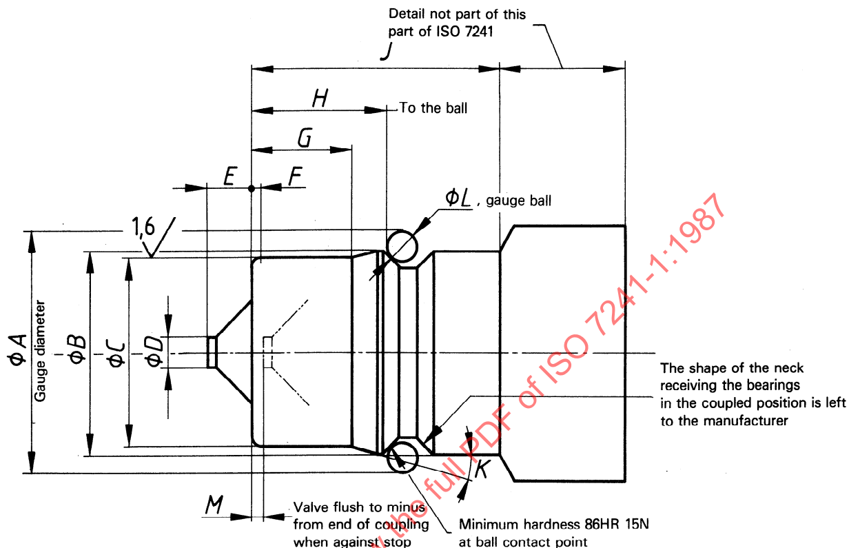
Figure 2 — Dimensional requirements, series "B" — Sizes 5 to 25
