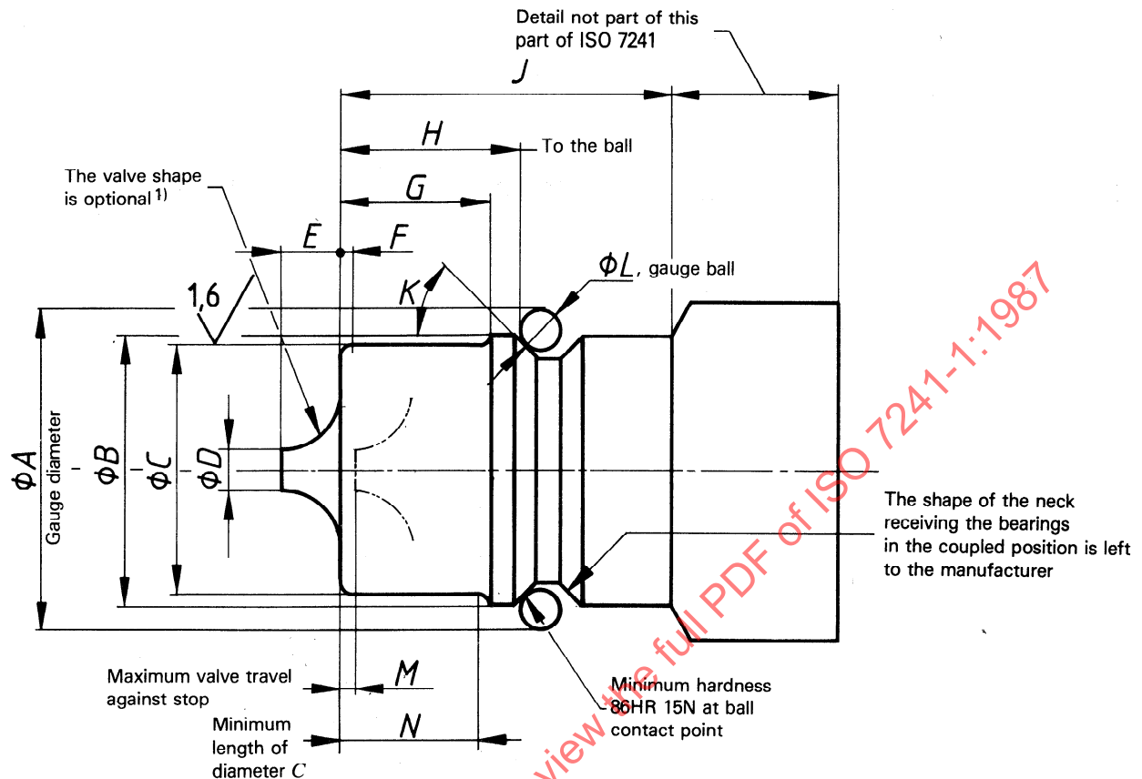
Figure 1 — Dimensional requirements, series "A"
