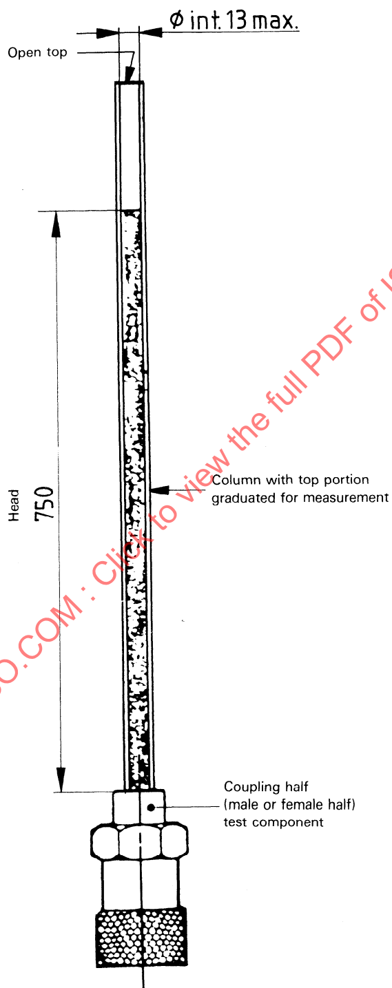
Figure 2 — Low-pressure leakage test apparatus (uncoupled half)
