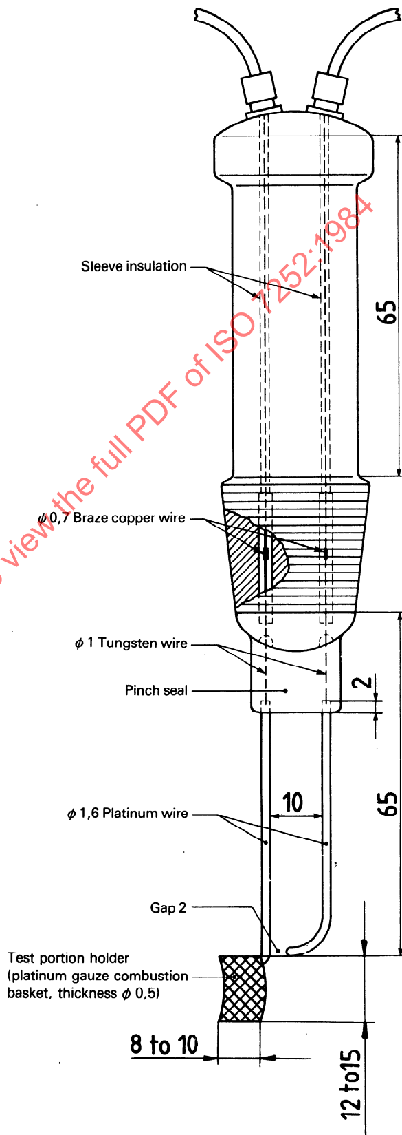
Figure 1 — Firing adapter
