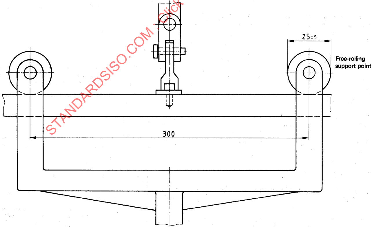
Figure 3 — Test fixture
