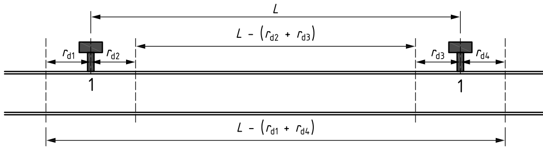
Figure 7 — Length between detectors
