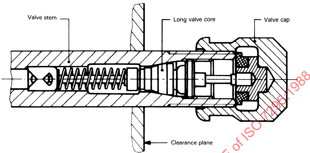
Figure 1 — General assembly for long core
