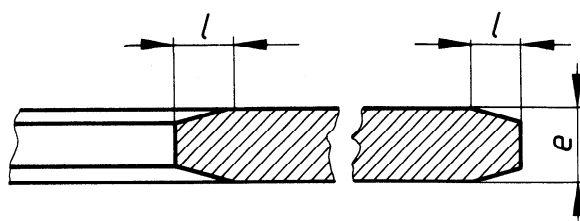
Figure 3 — Disk, edge chamfers, cross-sectional view
