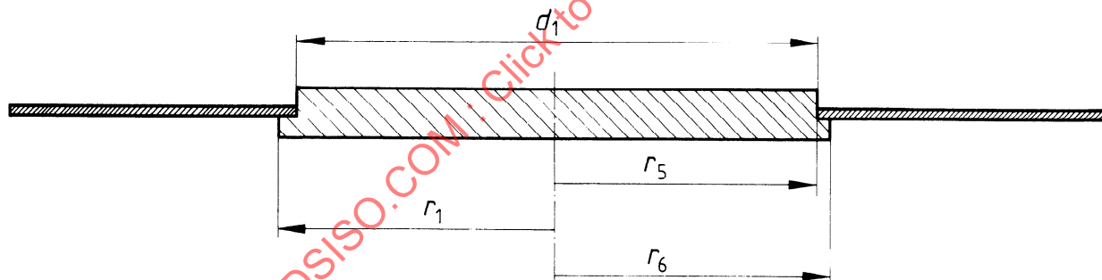
Figure 1 — Cross-sectional view of the reference hub with disk
