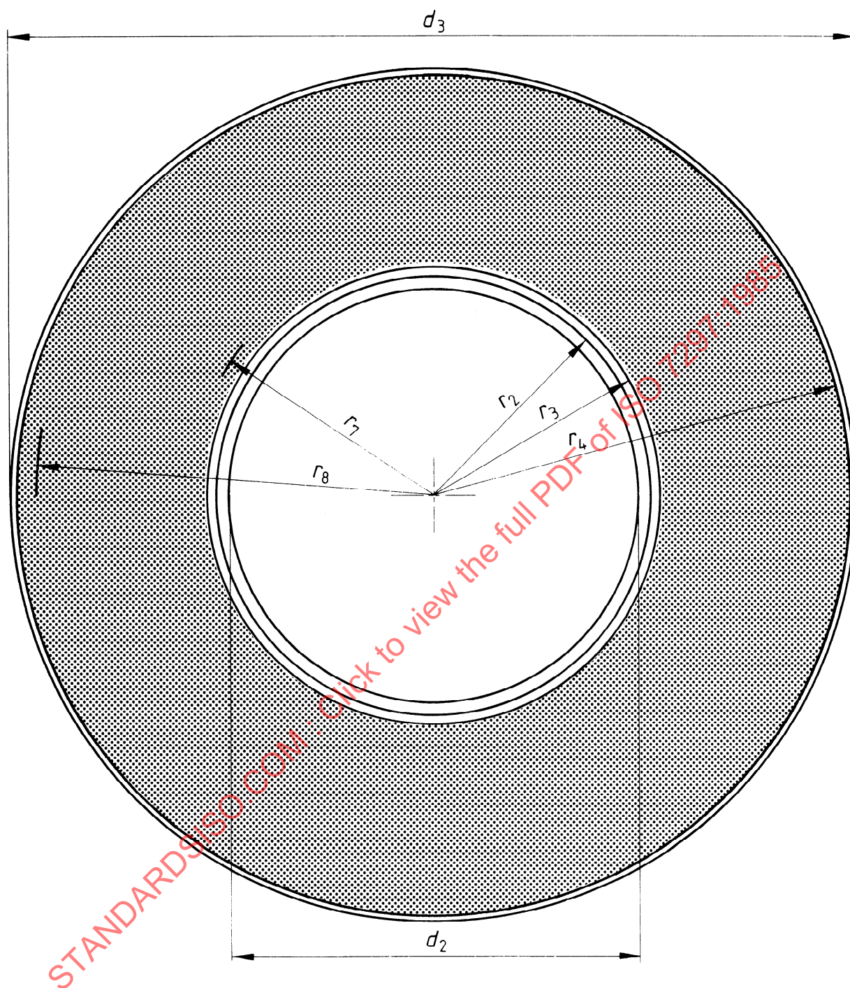
Figure 2 — Disk, top view
