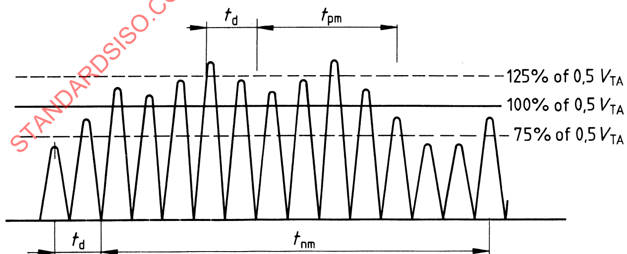
Figure 7 — Modulation tests
