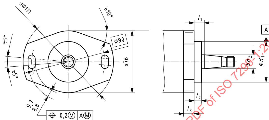
Figure 1 — Fuel injection pumps — Type 1 end-mounting flange
