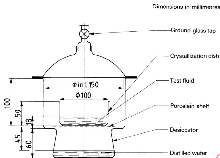
Figure 1 — Hygroscopicity apparatus
