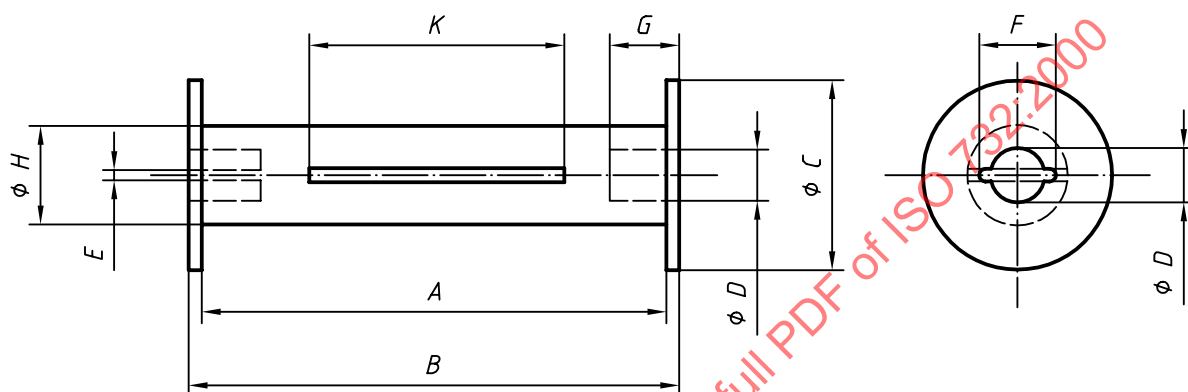
Figure 3 — Spool dimensions
