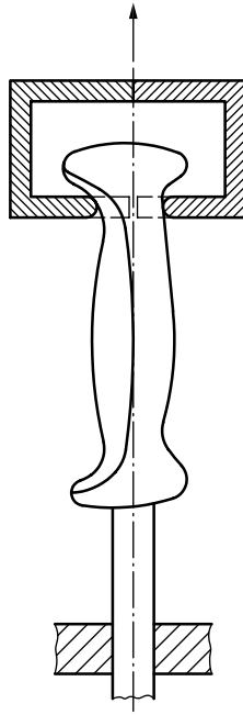
Figure 4 — Test arrangement for pulling-off force
