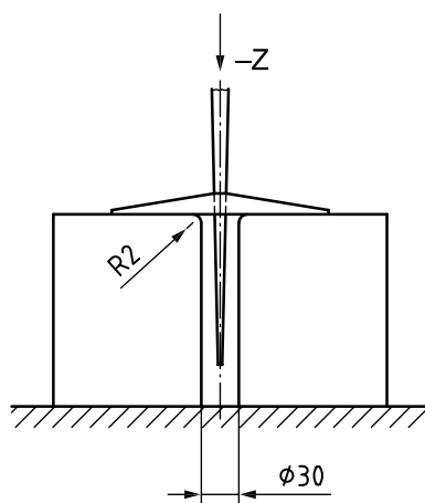
Figure 8 — Test arrangement for the basket and basket fixing in the direction of compression
