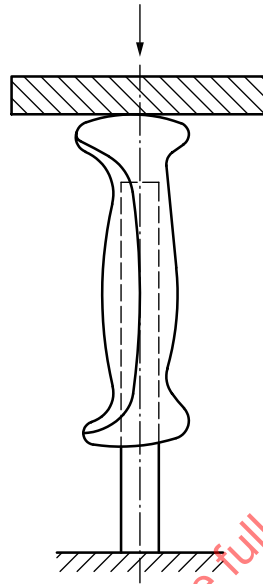
Figure 3 — Test arrangement for piercing resistance
