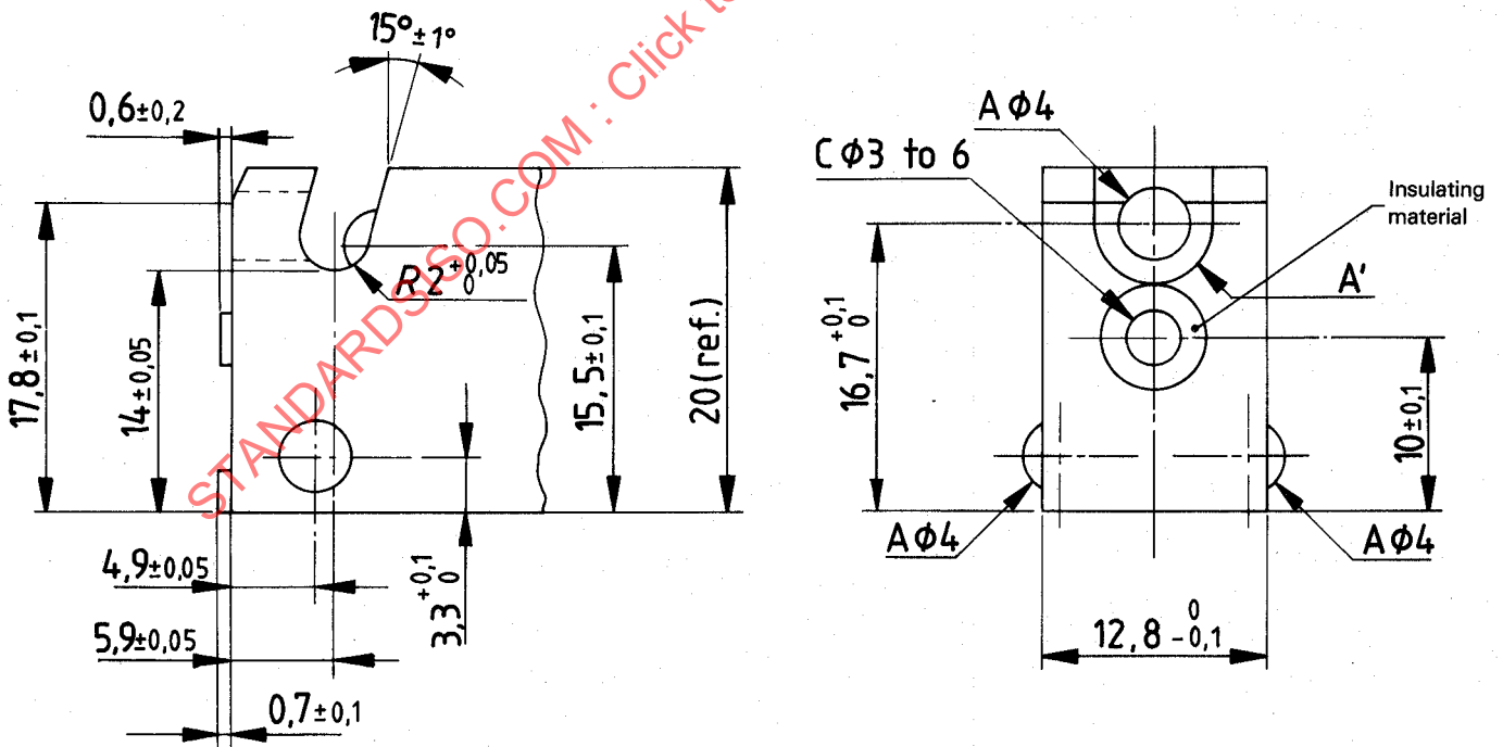
Figure 1a) — Blade hook-on fittings
