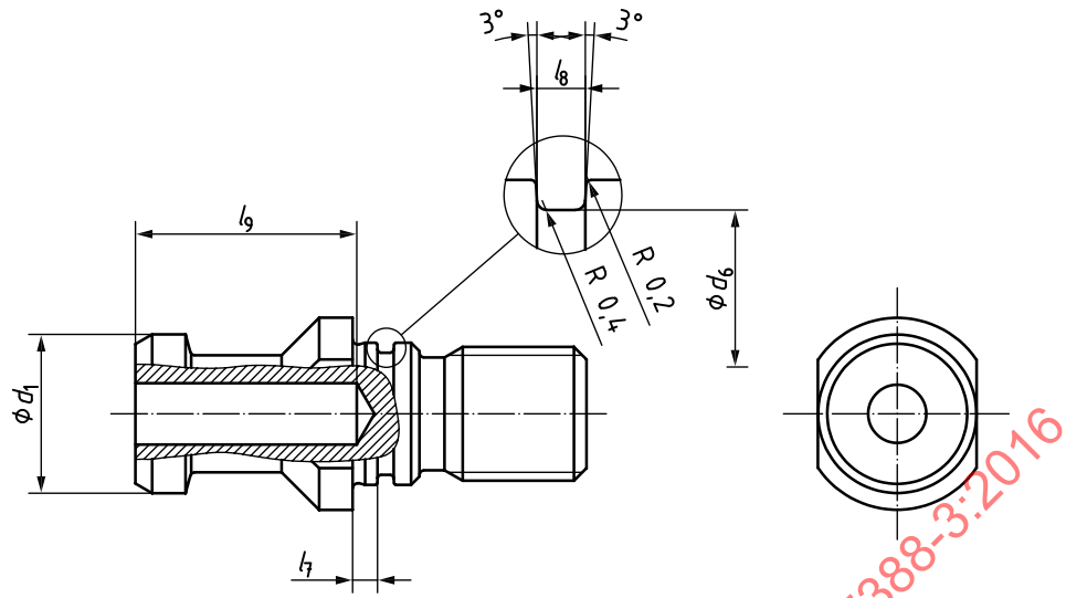
Figure 2 — Retention knob — Form AF — Without cooling lubricant supply
