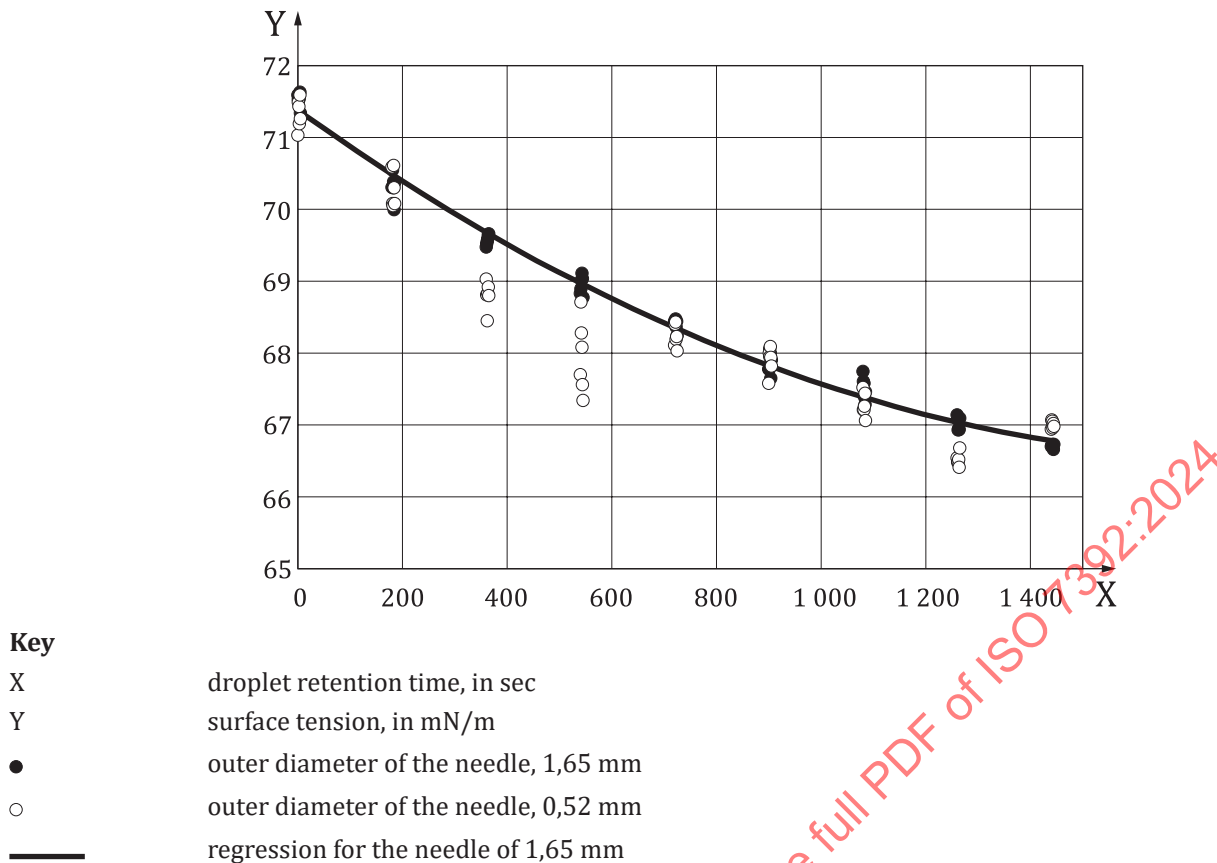
Figure B.5 — Dependence of the surface tension by the pendant drop method on the outer diameter of the needle
