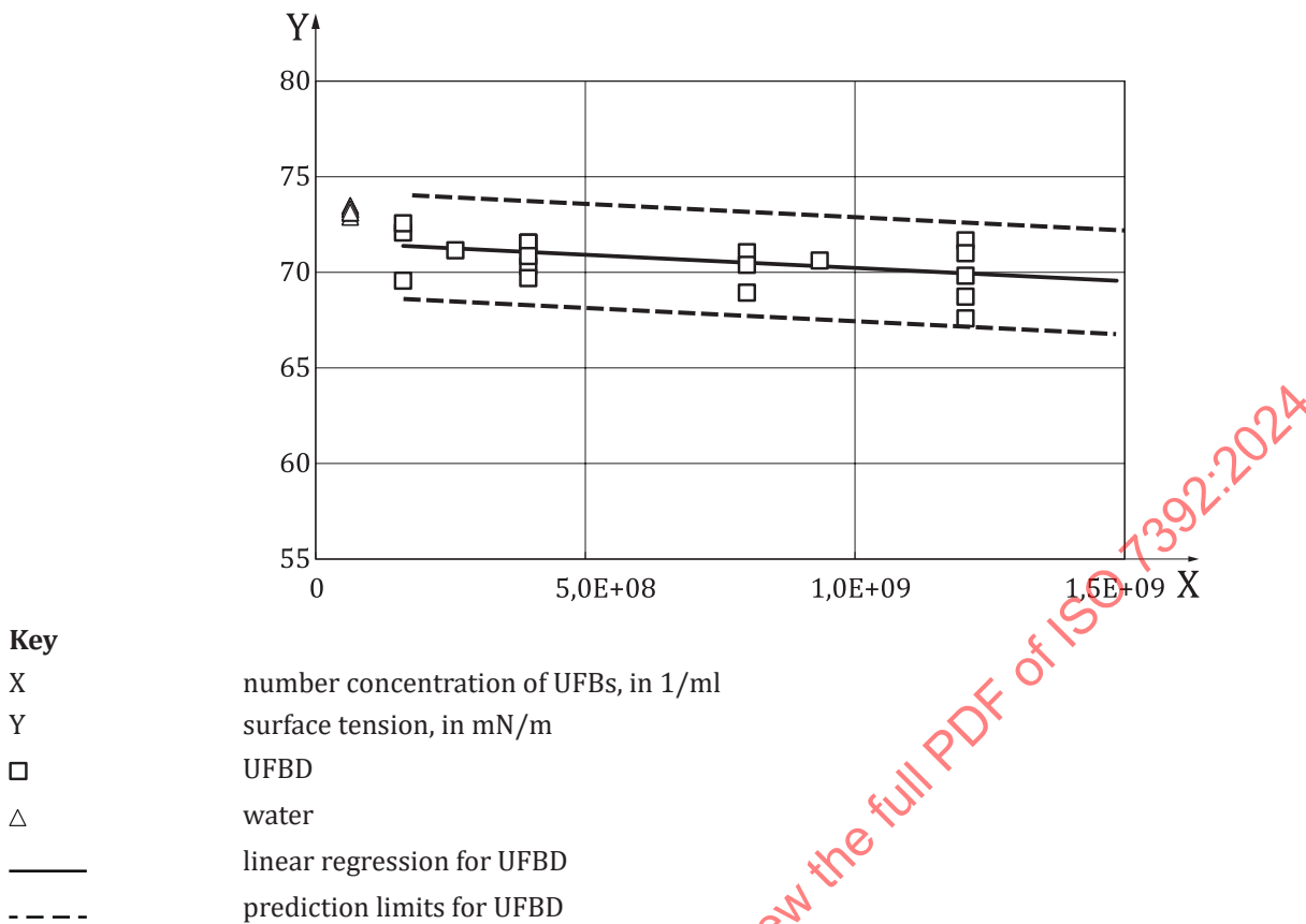
Figure B.2 — Surface tension of UFB dispersion of low concentration area (measurement results by the Wilhelmy method)
