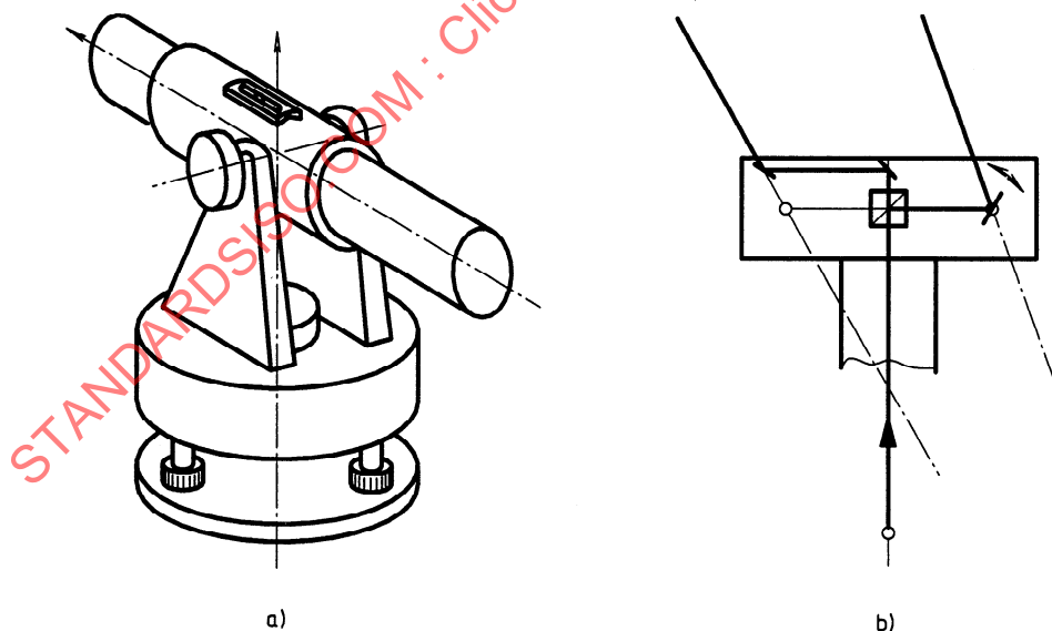
Figure A.1 — Typical axis system of theodolite
