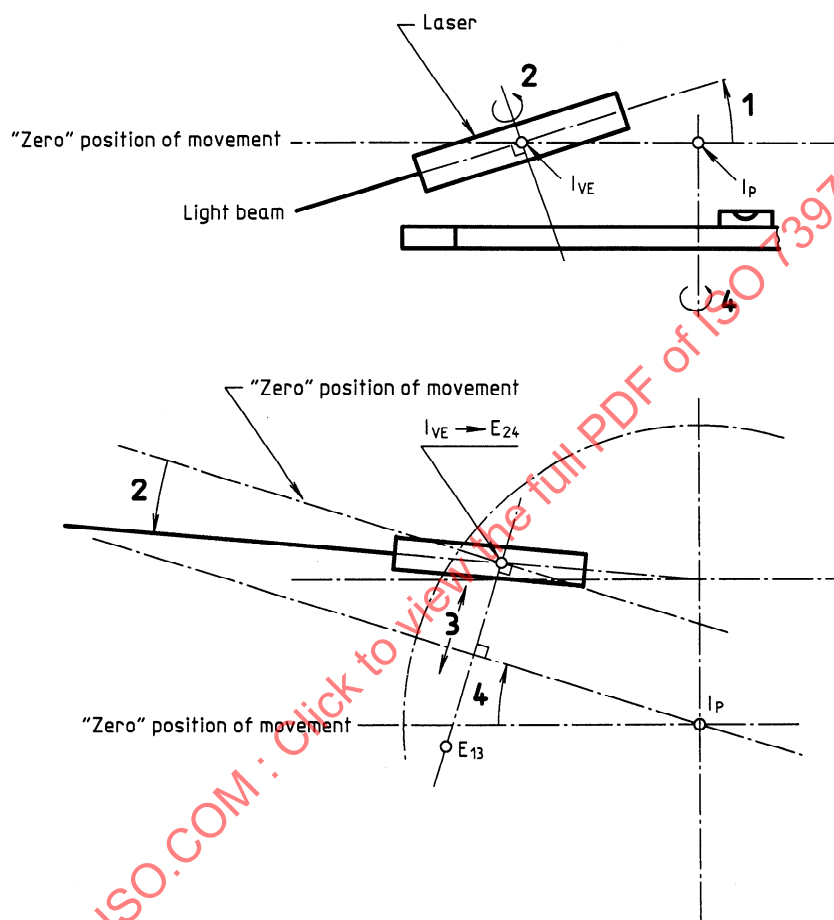
Figure A.2 — Laser device fitted on pivoting axis normal to fixed horizontal pivoting axis
