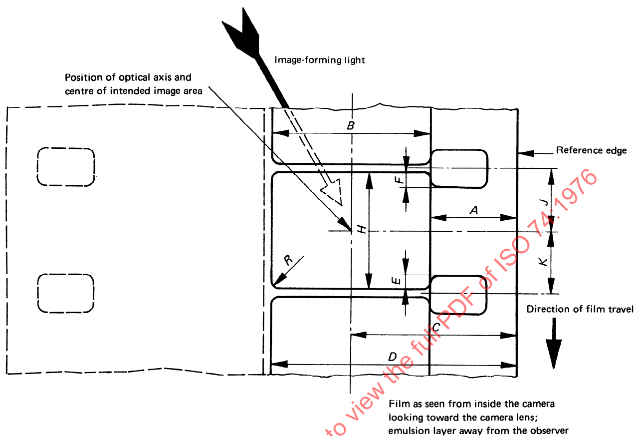
FIGURE 1 — Image area produced by camera aperture
