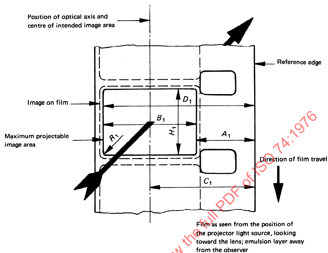
FIGURE 2 — Maximum projectable image area
