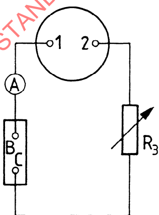
Figure 3 — Wiring diagram for overload strength test
