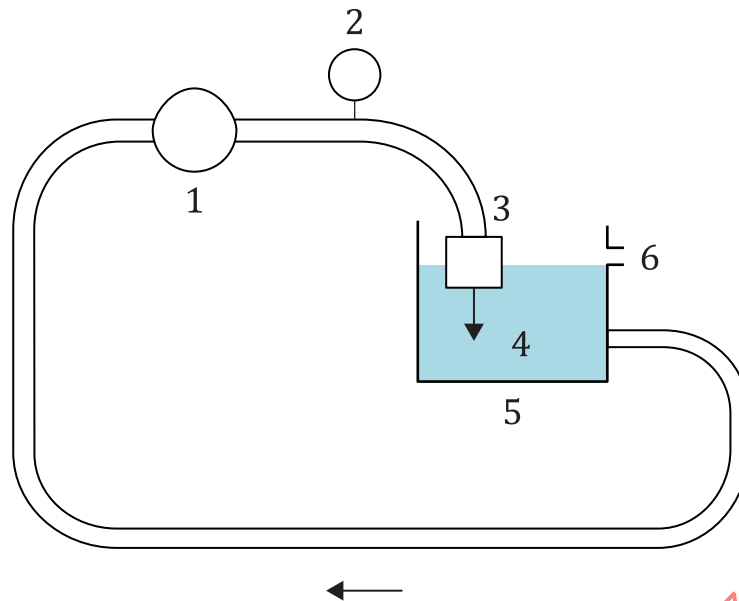
b) Submerged type of nozzle in retention container
