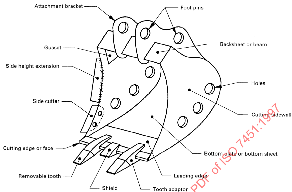
Figure 2 — Terminology of bucket components
