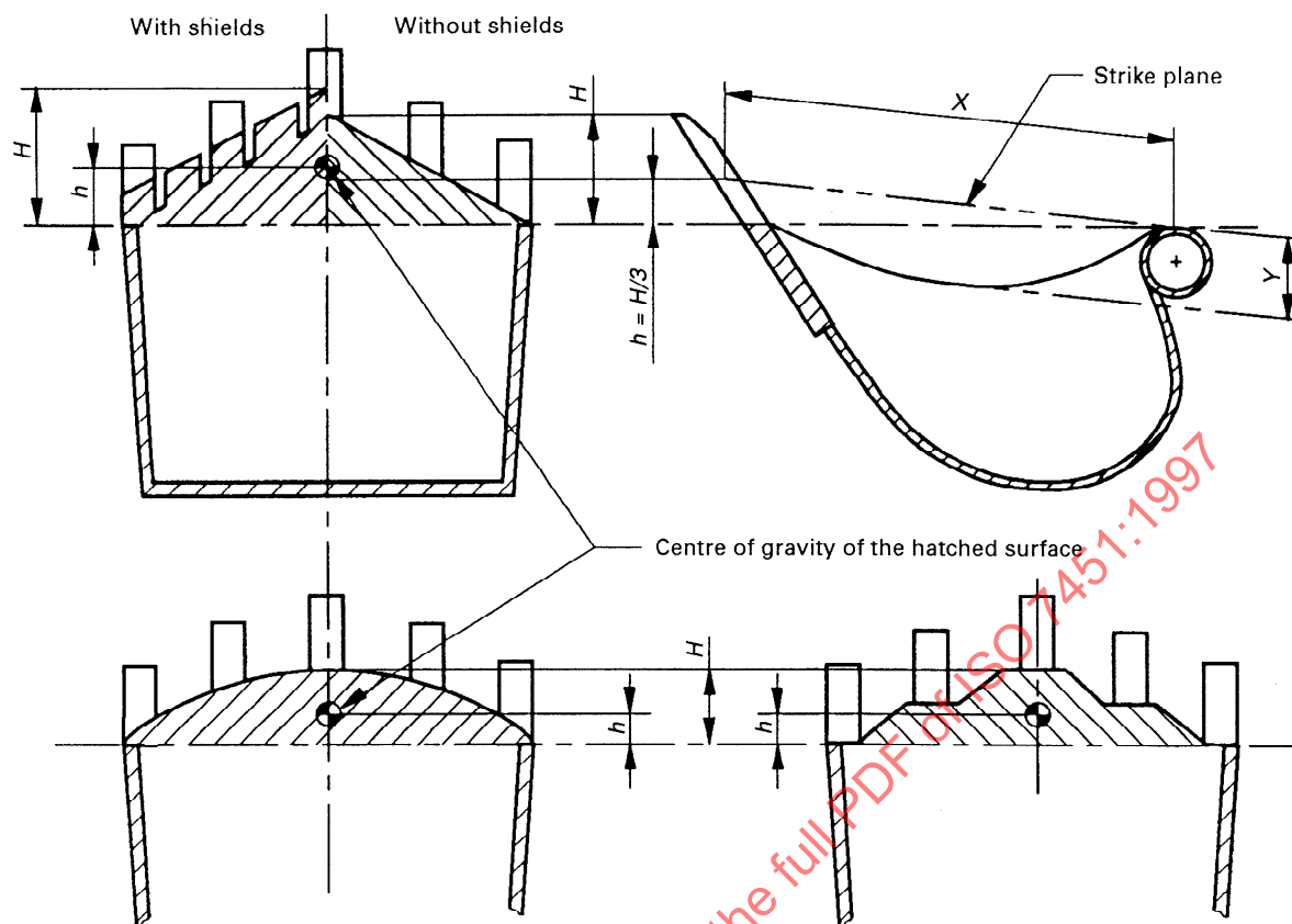
Figure 4 — Effect of leading edge shape on h value
