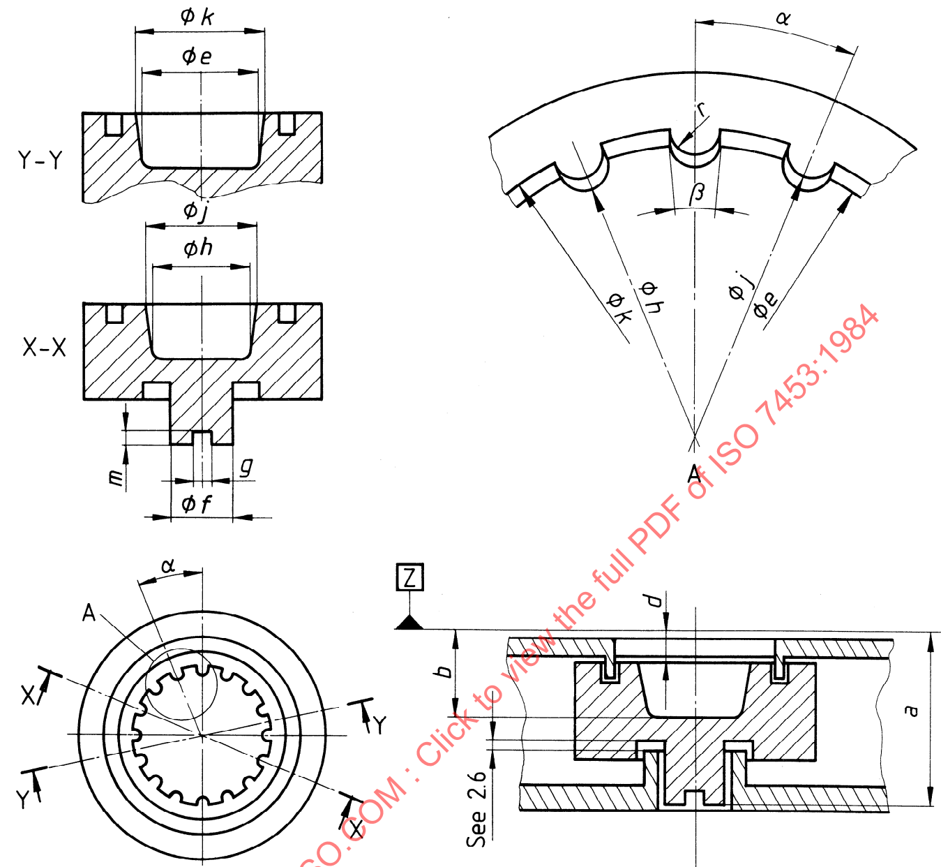
Figure 2 — Section of cartridge containing core (see 2.5)
