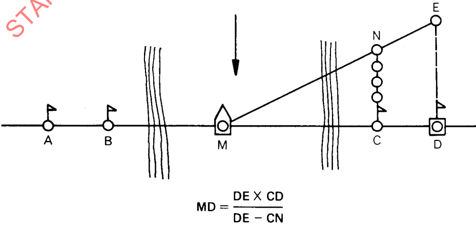
FIGURE 7 — Measurement of cross-section — Projection from one bank
