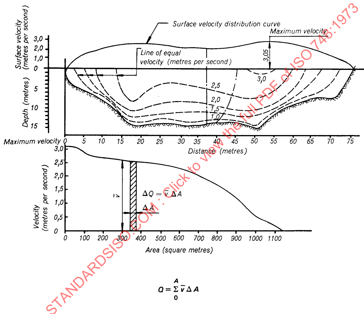
FIGURE 2 — Computation of discharge from current-meter measurements — Area-velocity integration method
