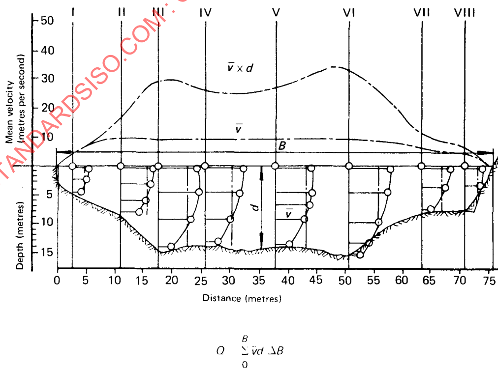
FIGURE 1 — Computation of discharge from current-meter measurement — Depth-velocity integration method
