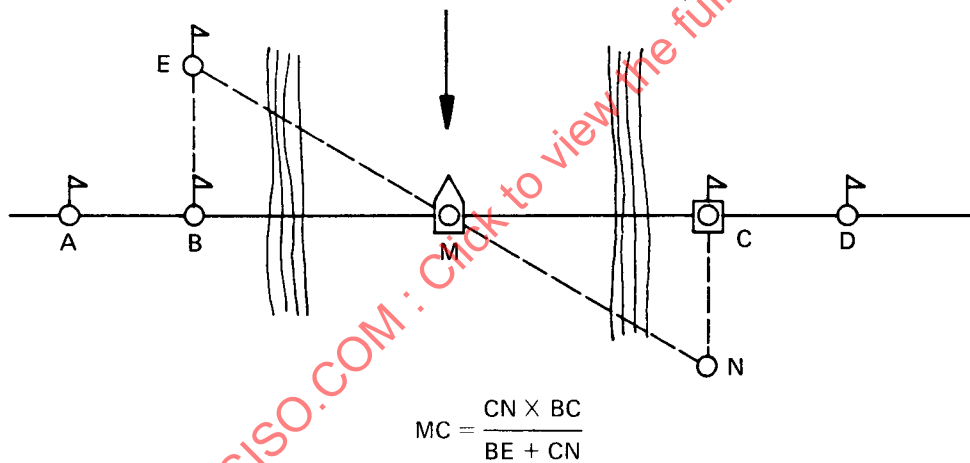
FIGURE 6 — Measurement of cross-section — Projection from opposite bank
