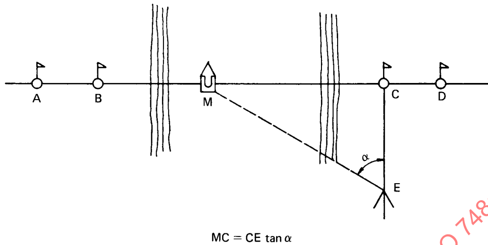
FIGURE 5 — Measurement of cross-section — Angular method
