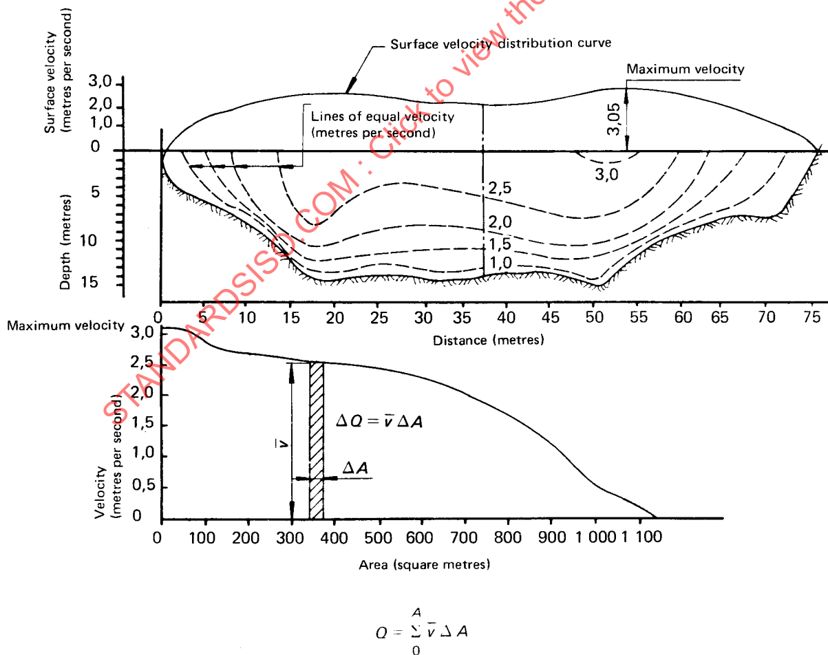
FIGURE 2 — Computation of discharge from current-meter measurement — Area-velocity integration method
