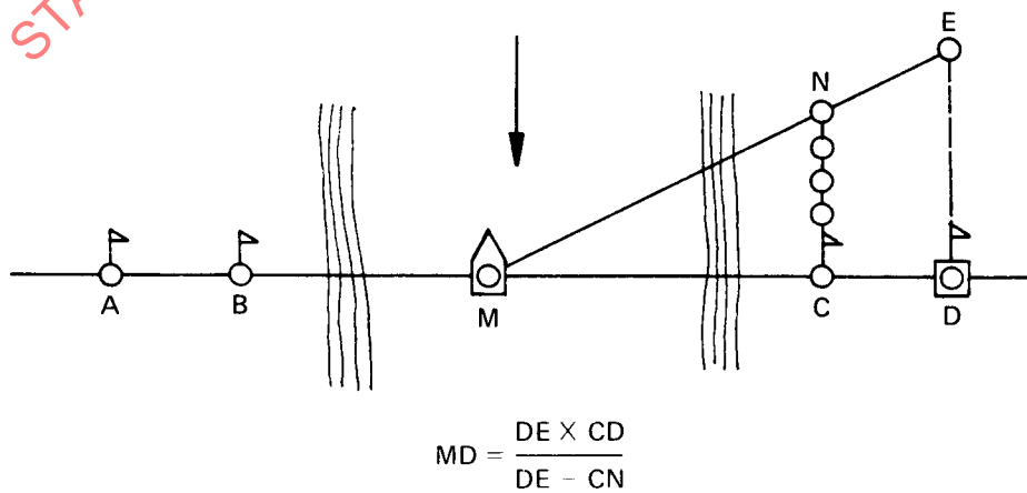
FIGURE 7 — Measurement of cross-section — Projection from one bank
